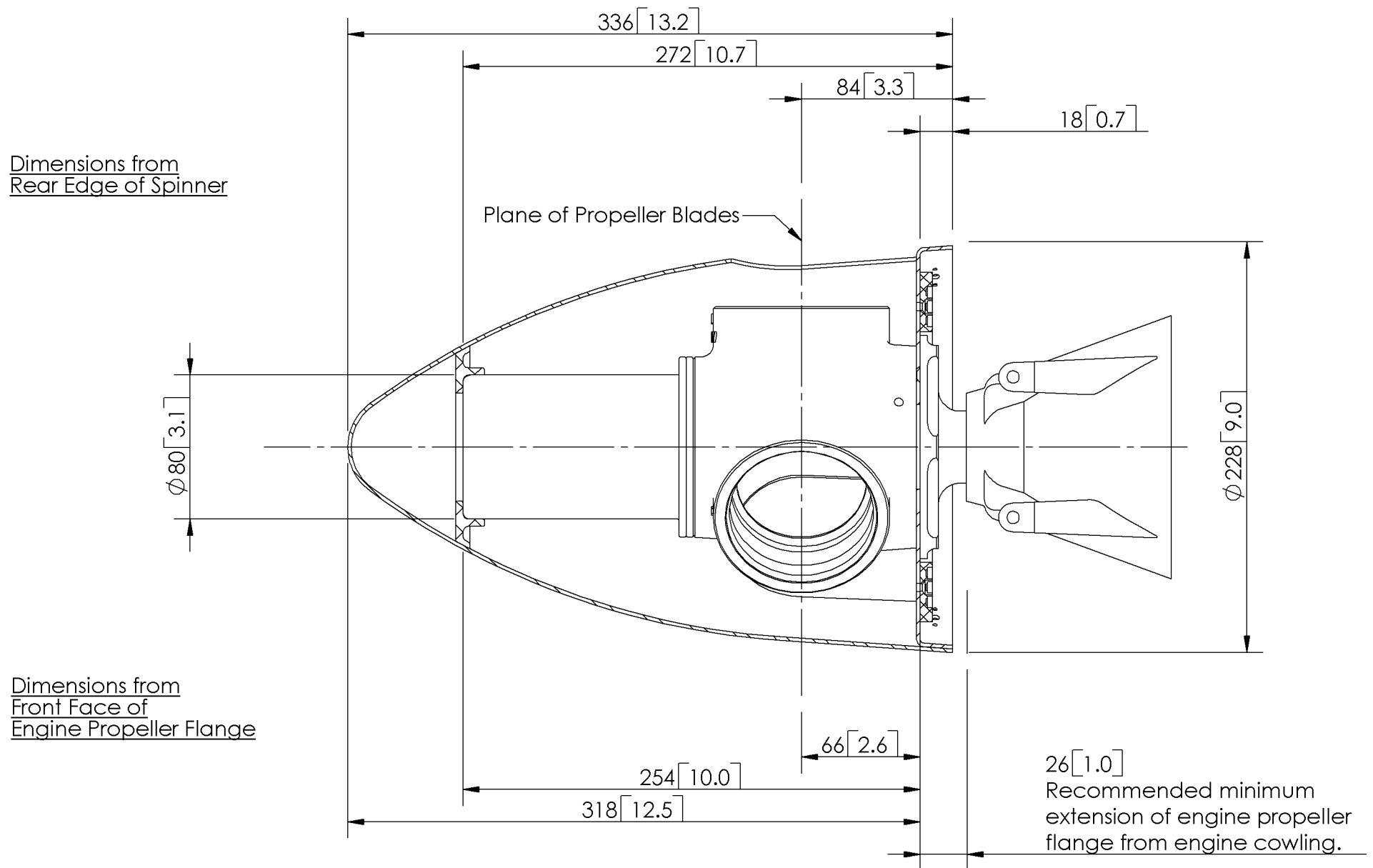
Principal Dimensions of AP332 Propeller with \phi 228\text{mm} (9in) Spinner (Example shown mounted on Rotax engine) Primary dimensions in millimeters [secondary dimensions in inches]
